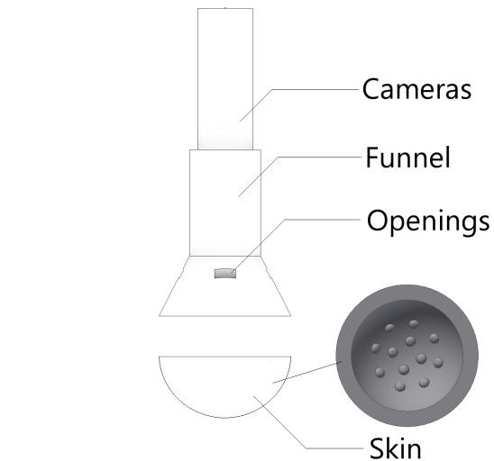
Fig. 1. Layout of the sensor.
