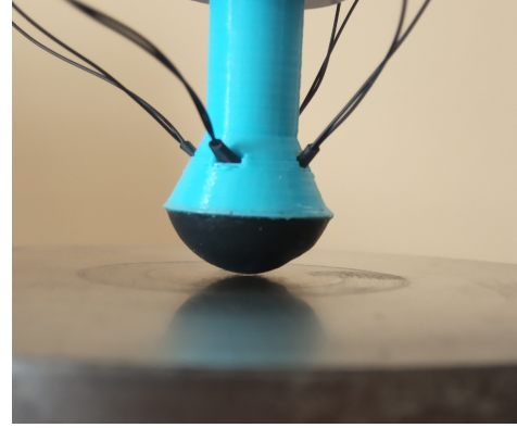
Fig. 3. Sensor before contact.
