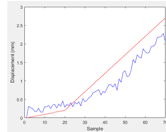
Fig. 4. Displacement per sample for the first two experiments. The red line represents the experimental data, and the blue line shows the results obtained from the sensor
